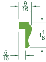
#292 WAINSCOT CAP 1-1/8"Hx9/16"D
