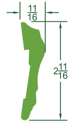
#390 CHAIR RAIL 2-11/16"Hx11/16"D
