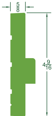
#2203 FLAT JAMB CRAFTSMAN STOP 4-9/16"Hx5/8"D
