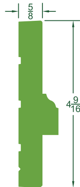
#2202 FLAT JAMB COLONIAL STOP 4-9/16"Hx5/8"D
