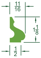
#164 BASE CAP 1-1/8"Hx11/16"D
